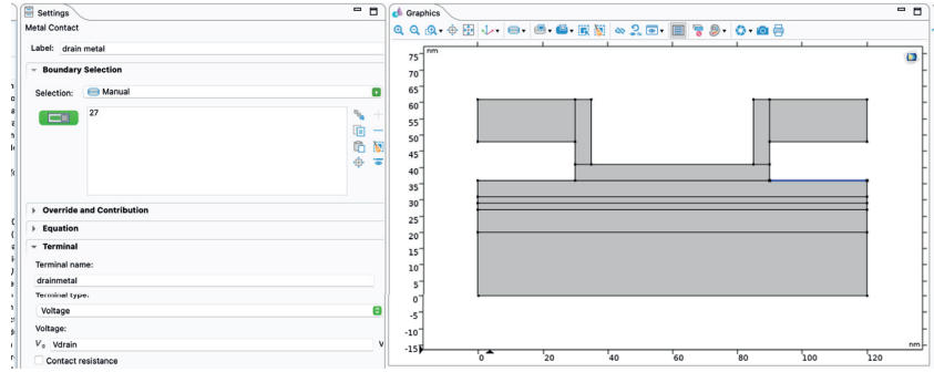
Figure 3.7: Ohmic metal contact with voltage V_{drain} for the drain.
