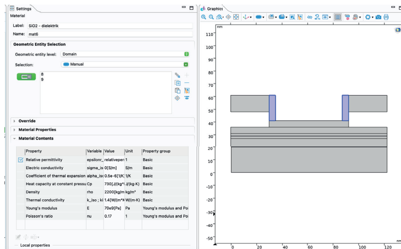
Figure A.22: SiO 2 dielectric domains.
