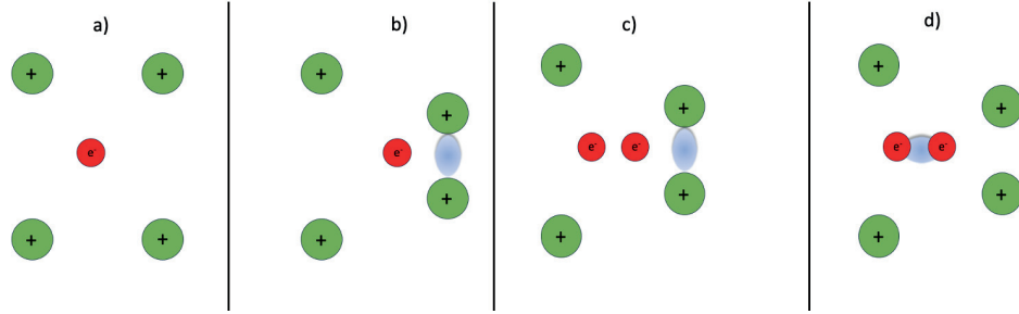
Figure 2.1: Schematic illustration of phonon-mediated electron pairing. (a) An electron moving through the lattice. (b) The electron attracts nearby positive ions, creating a local lattice distortion. (c) The resulting region of increased positive charge can attract a second electron. (d) The two electrons form a bound Cooper pair [10].
