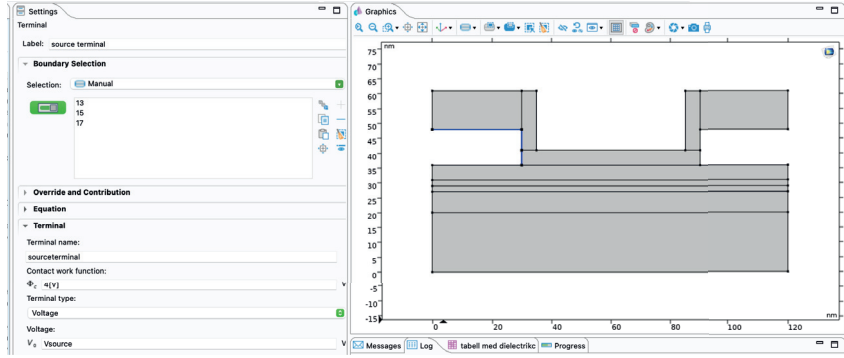
Figure 3.6: The source terminal with voltage V_{source} .
