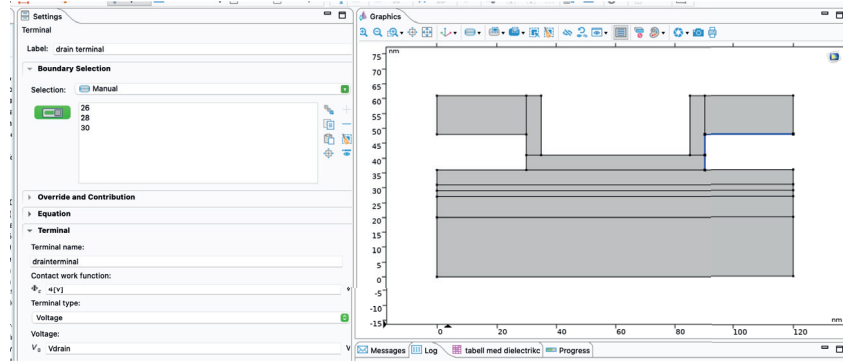
Figure 3.8: The drain terminal with voltage V_{drain} .
