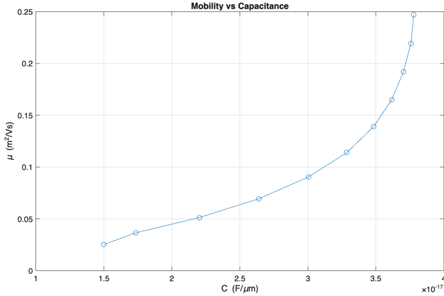
Figure 4.19: Mobility \mu as a function of capacitance.
