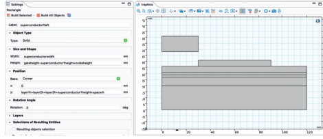
Figure A.13: The left air region.
