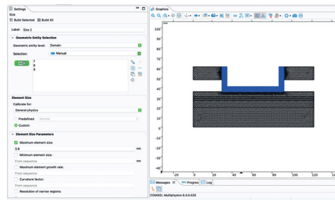
Figure A.38: Finer mesh applied to the dielectric and oxide domains.
