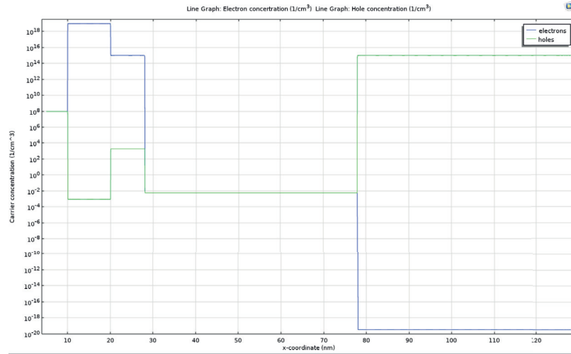
Figure 4.15: Electron and hole concentration along the growth direction.
