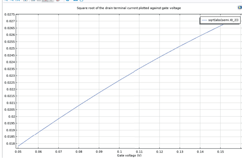
Figure 4.2: Linear region of the \sqrt{I_D} - V_{gate} characteristic used for threshold voltage extraction. The highlighted interval shows the portion of the curve exhibiting approximately linear behavior and used for the linear fit.
