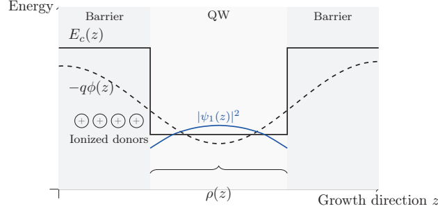
Figure 2.4: Schematic conduction band edge E_c(z) and electrostatic potential -q\phi(z) in a quantum well heterostructure, including the ground-state wavefunction |\psi_1(z)|^2 representing the 2DEG distribution.
