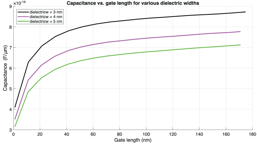
Figure 4.5: Capacitance varying with gate length and dielectric width for three different widths of the dielectrics.
