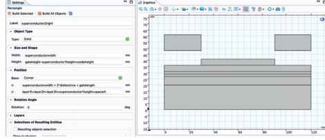
Figure A.14: The right air region.
