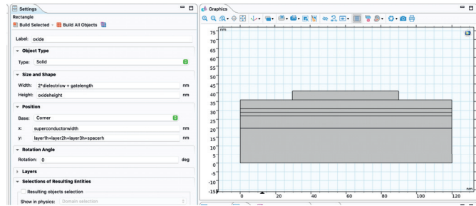
Figure A.12: The oxide layer.
