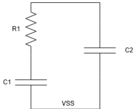
Figure 2.7: typical passive 2nd LPF
