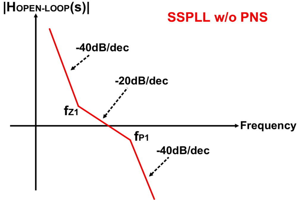
Figure 3.11: Conceptual open-loop gain of Conventional SSPLL [4]
