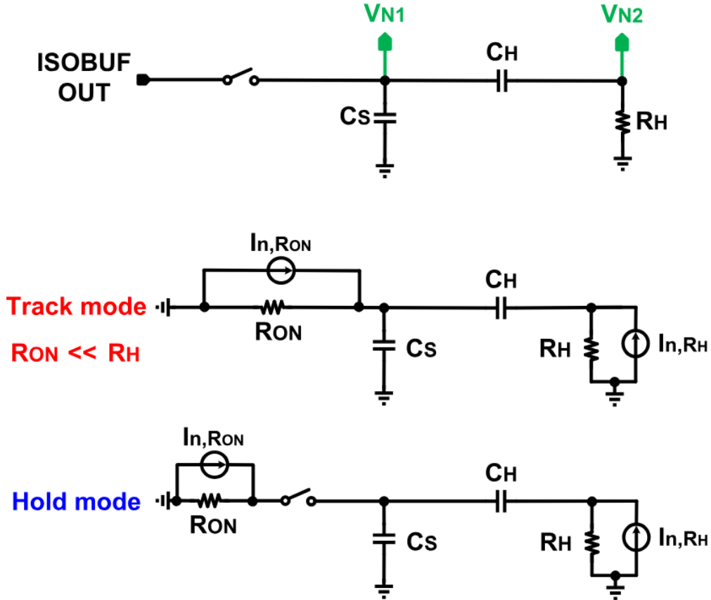
Figure 3.13: Noise analysis of the SSPD and HPF [4]
