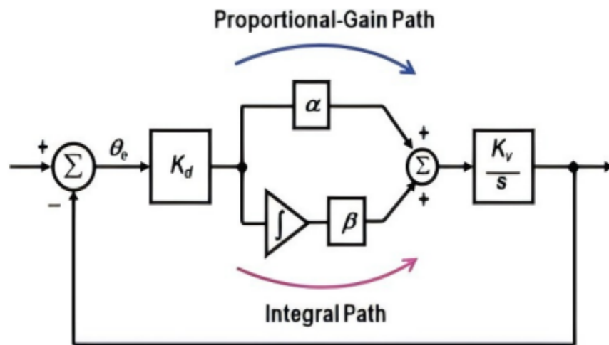
Figure 2.6: Two paths for LPF [10]
