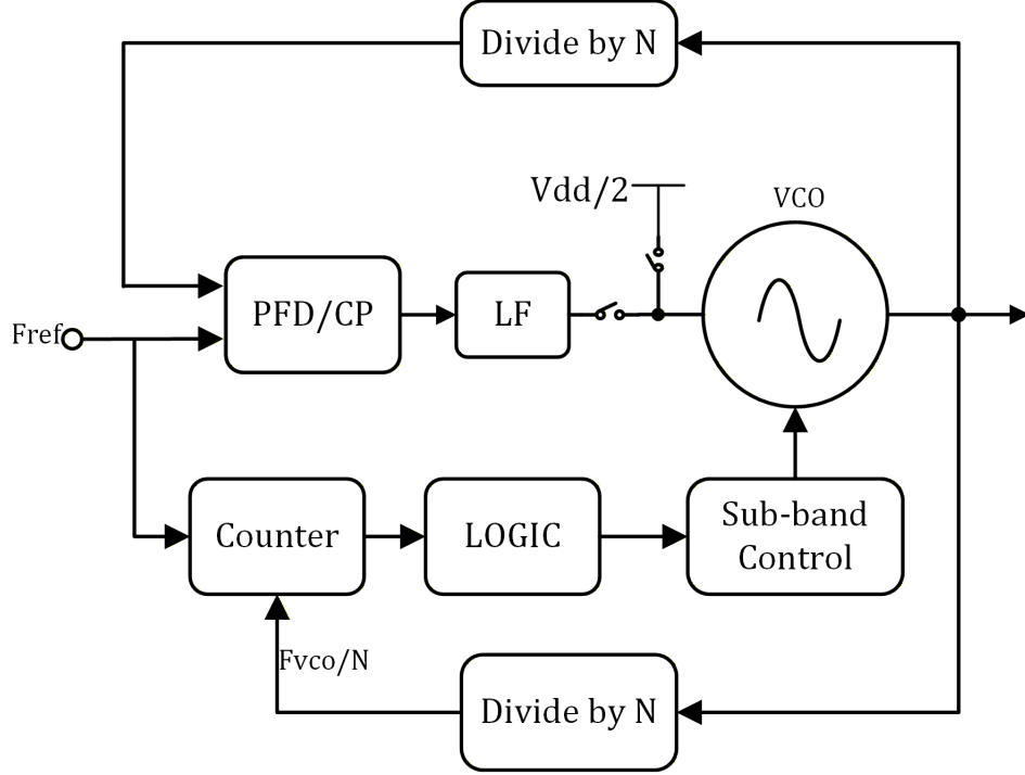
Figure 3.16: Conventional open-loop VCO calibration technique
