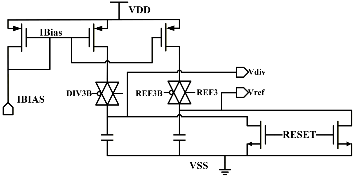
Figure 4.13: Circuit Design of the TVC
