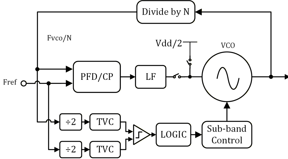
Figure 3.17: TVC-based agile VCO calibration technique
