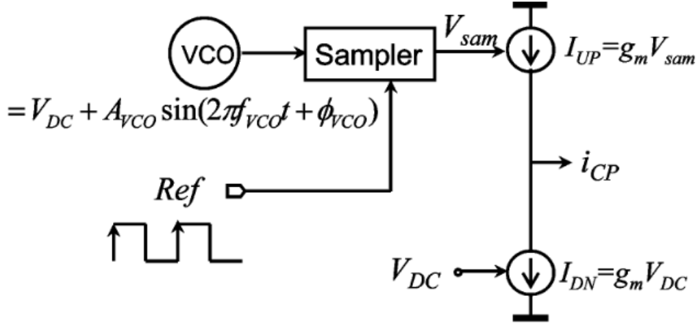
Figure 3.4: Conceptual diagram of SSPD/CP [3]
