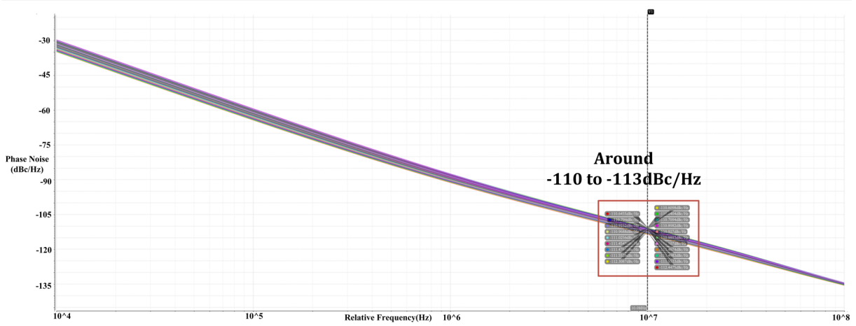
Figure 5.5: Phase noise performance of free-running VCO
