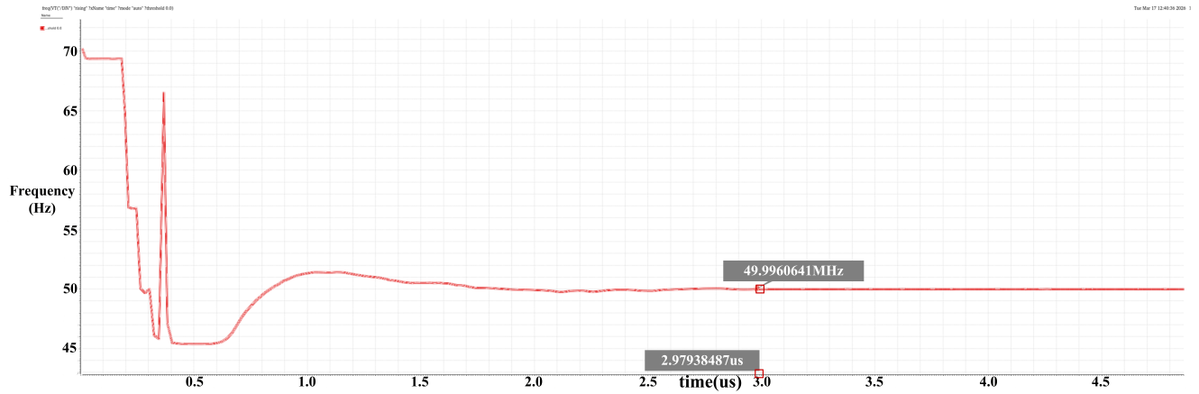
Figure 5.11: Transient behavior of the divided output signal
