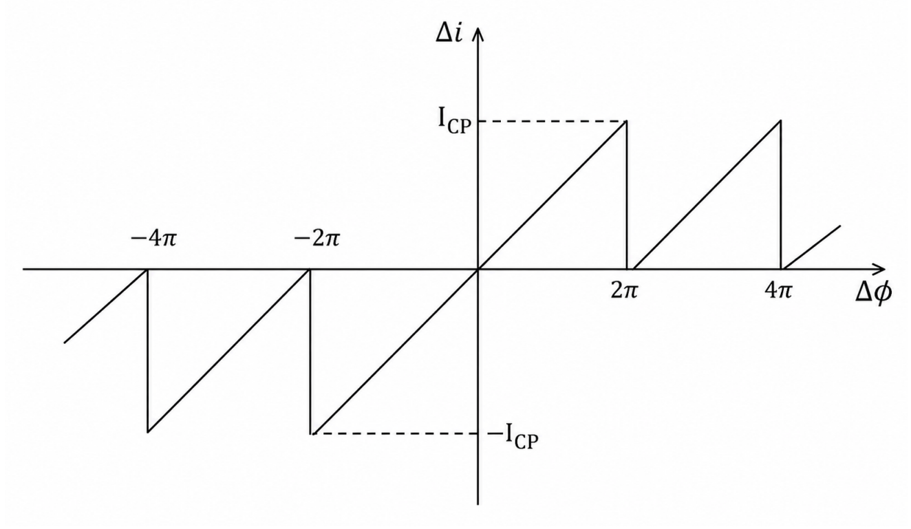
Figure 2.4: PFD/CP characteristics
