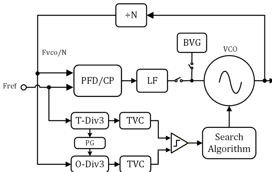
Figure 3.20: Block diagram of the proposed AFC
