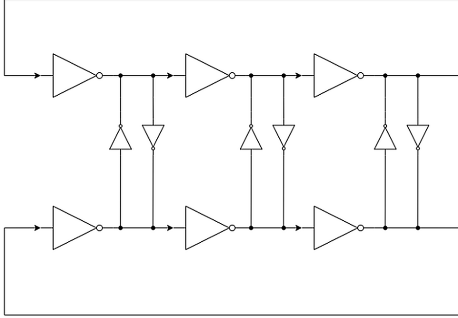
Figure 4.7: Block diagram of the ring VCO
