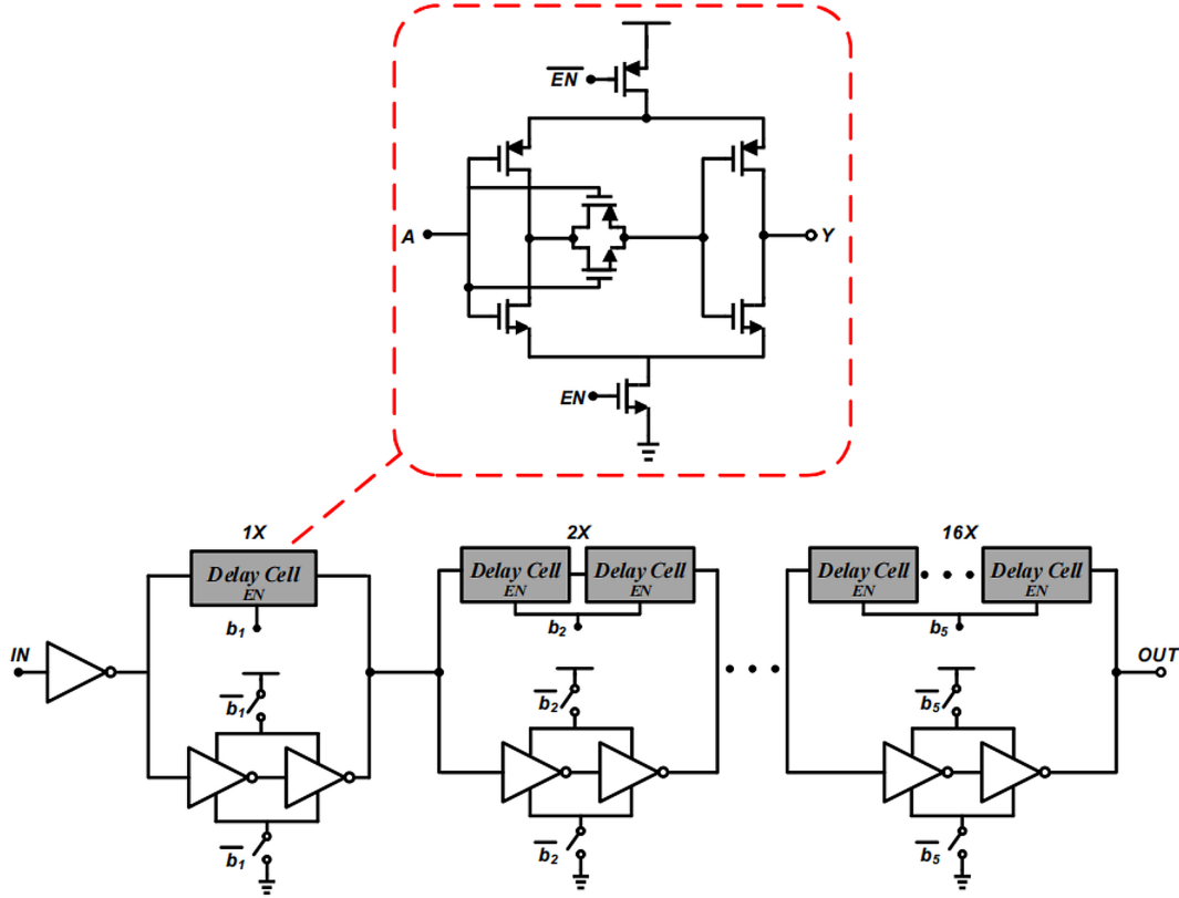
Figure 4.4: Circuit design of the Pulser control unit
