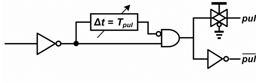
Figure 4.3: Circuit design of the Pulser
