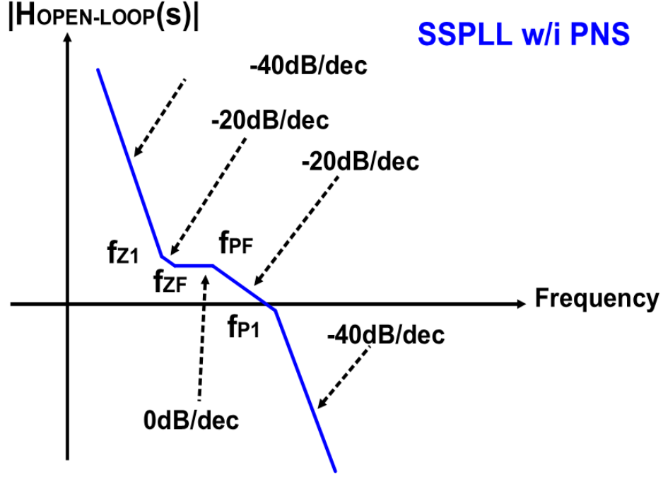
Figure 3.12: Conceptual open-loop gain of Dual-path SSPLL [4]
