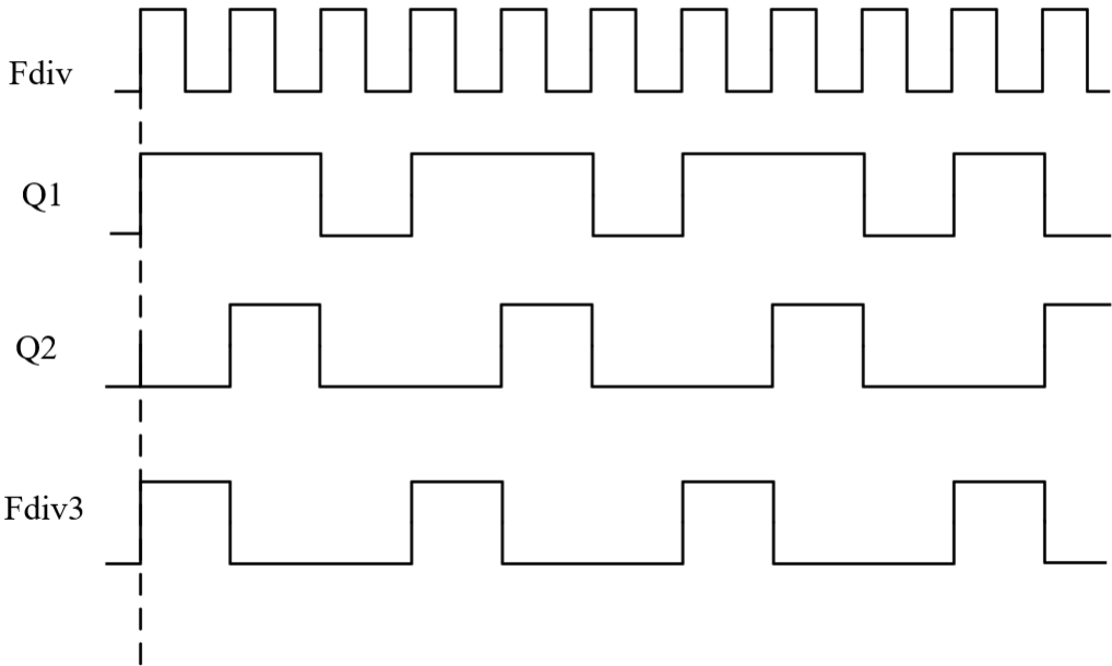
Figure 3.24: Q1Q2='00'
