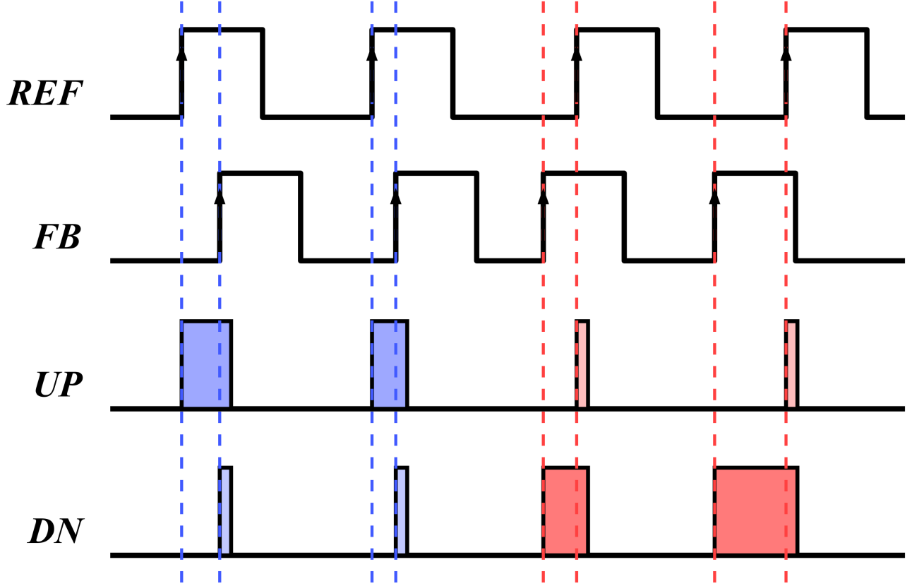
Figure 2.3: timing diagram of a tri-state PFD
