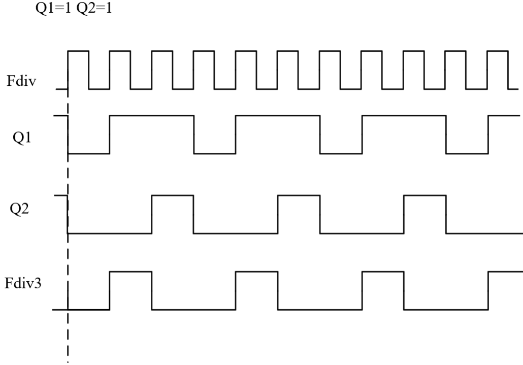
Figure 3.23: Q1Q2='11'
