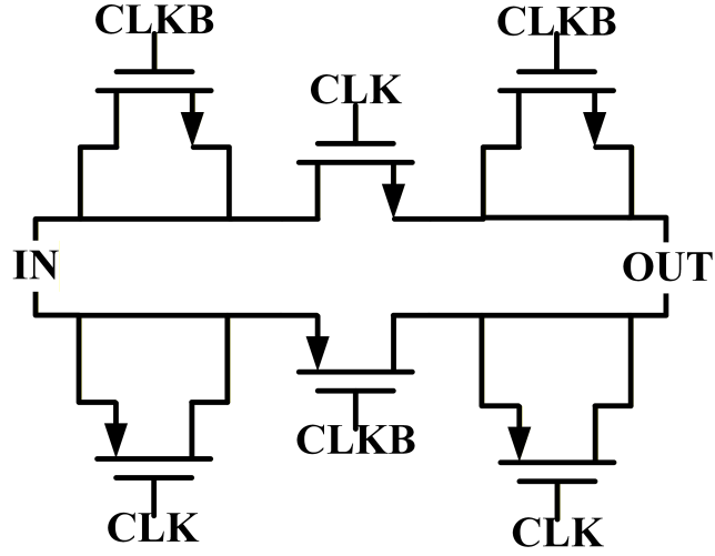
Figure 4.14: Circuit Design of the switch in TVC
