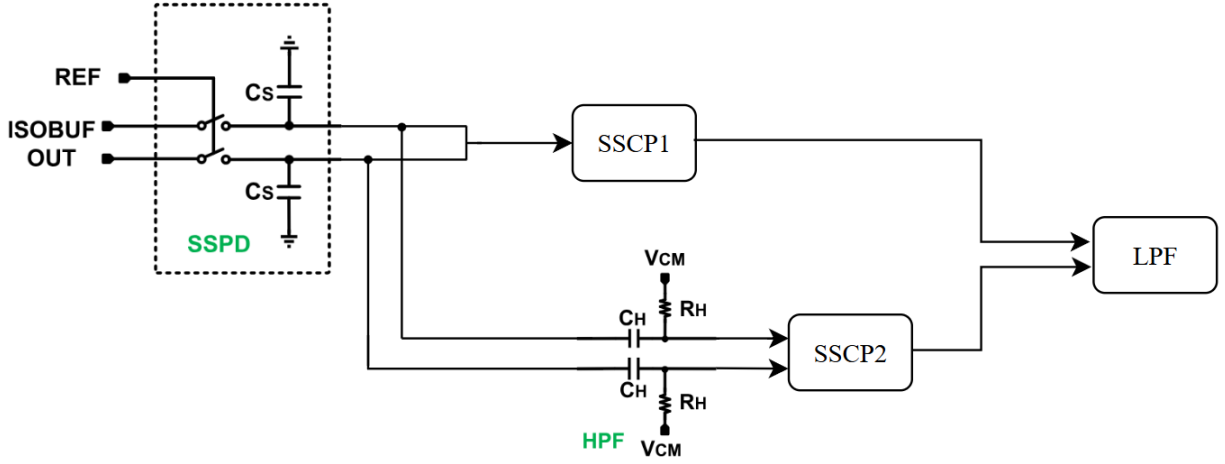
Figure 3.10: Circuit implementation of the HPF
