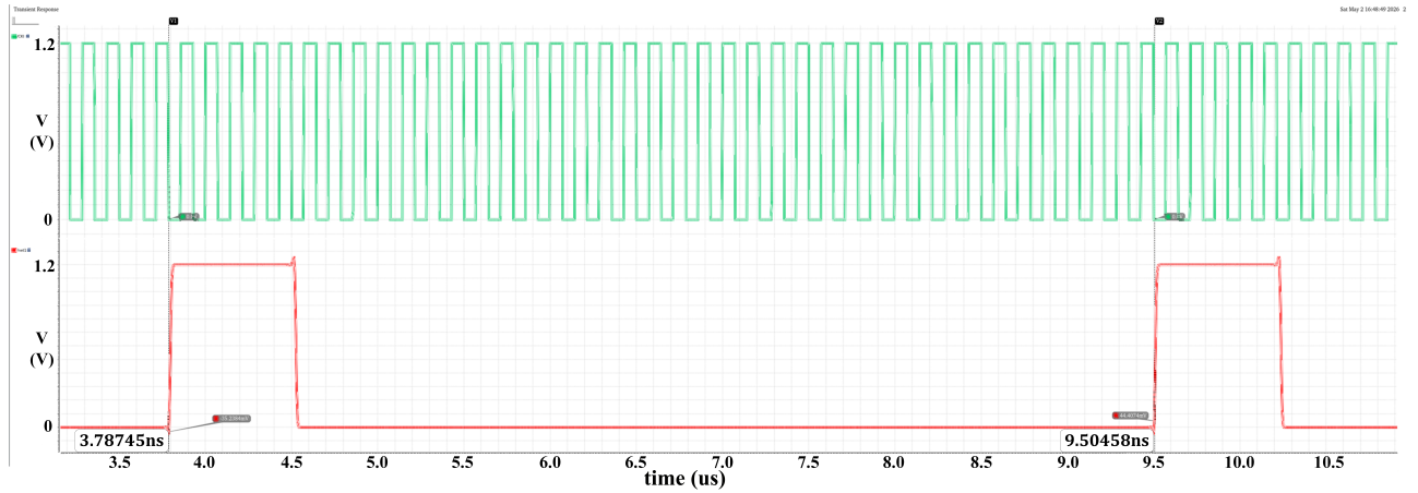
Figure 5.7: Transient simulation of the divider
