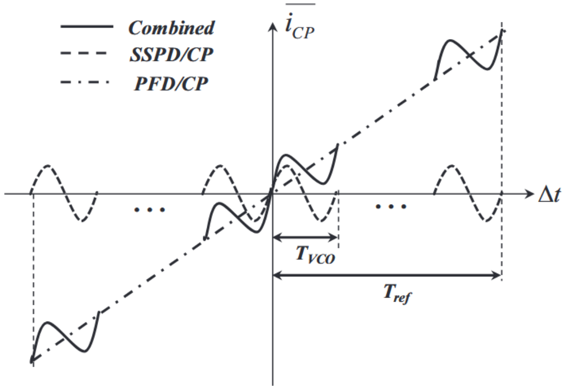
Figure 3.8: Combined SSPD/CP and PFD/CP characteristic [14]
