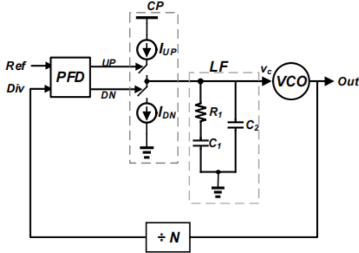
Figure 2.1: loop diagram of a CPPLL
