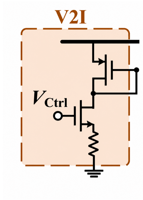
Figure 4.6: V2I converter in VCO. [20]
