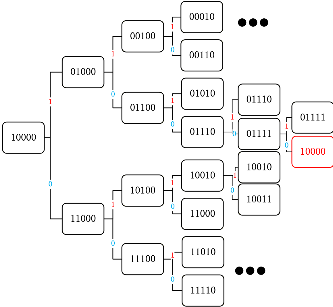
Figure 3.28: Switching scheme of the proposed O-AFC.
