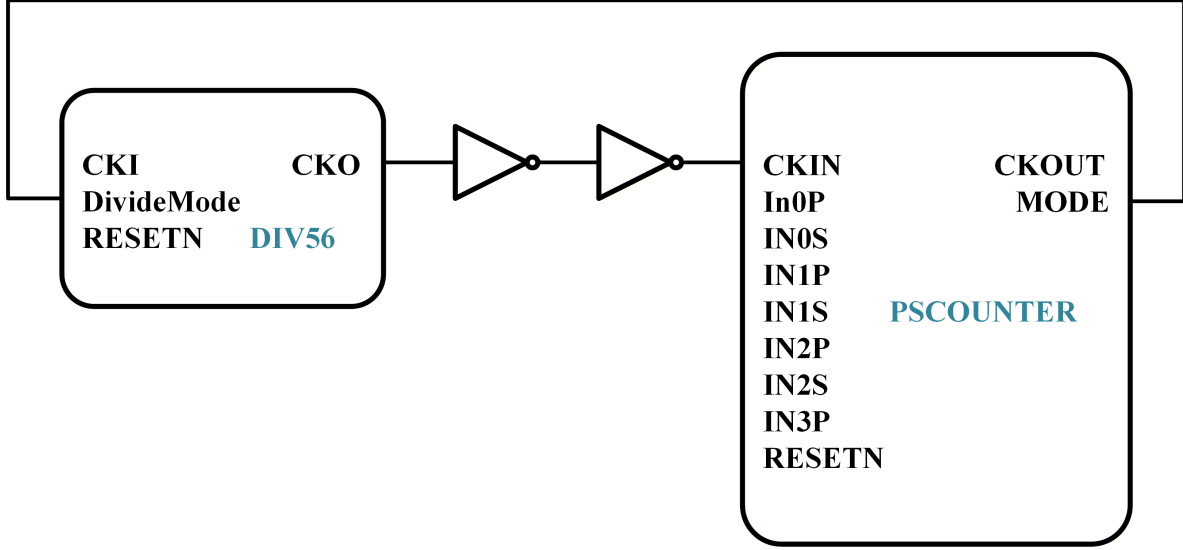
Figure 4.10: Block Diagram of the Prescaler
