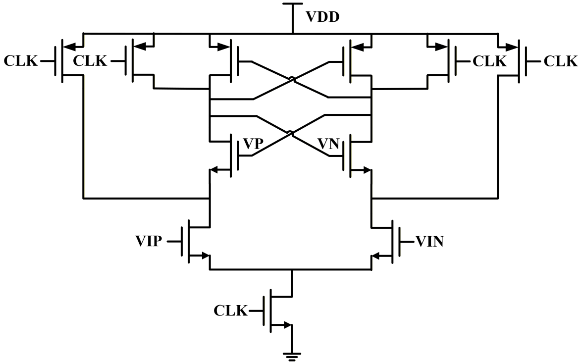
Figure 4.15: Circuit Design of the Comparator
