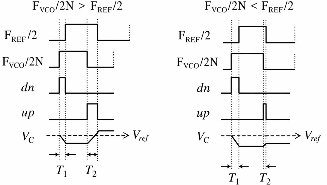
Figure 3.19: Operation timing diagram of the relative measurement
