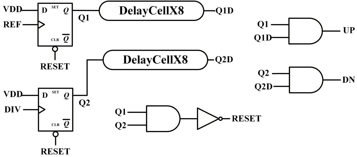
Figure 4.9: Circuit design of the PFD with DZ
