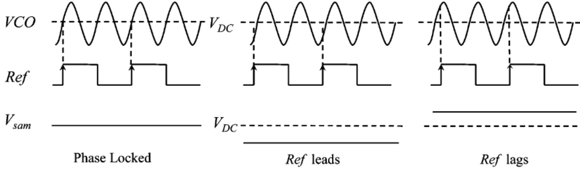
Figure 3.3: Timing diagram of sampling based PD [3]
