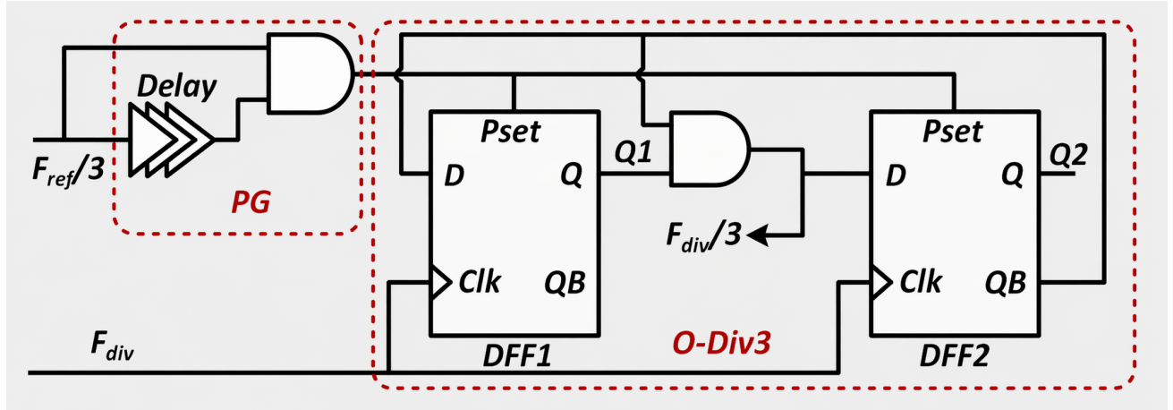
Figure 3.21: Implementation of O-Div3 circuit [18]
