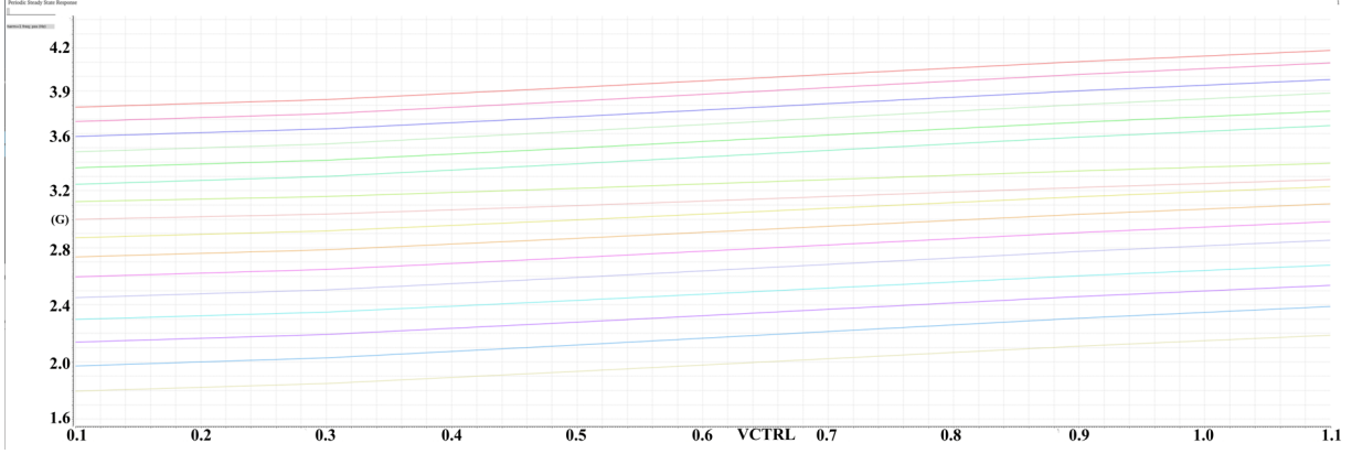
Figure 5.4: VCO sub-bands
