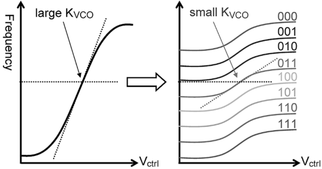
Figure 3.14: Technique for reducing the VCO tuning gain [17]
