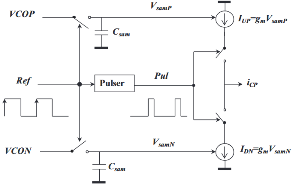
Figure 3.6: SSPD/CP with pulser gain control [14]
