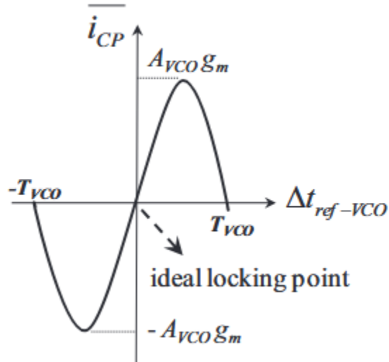
Figure 3.5: Characteristic of SSPD/CP [14]
