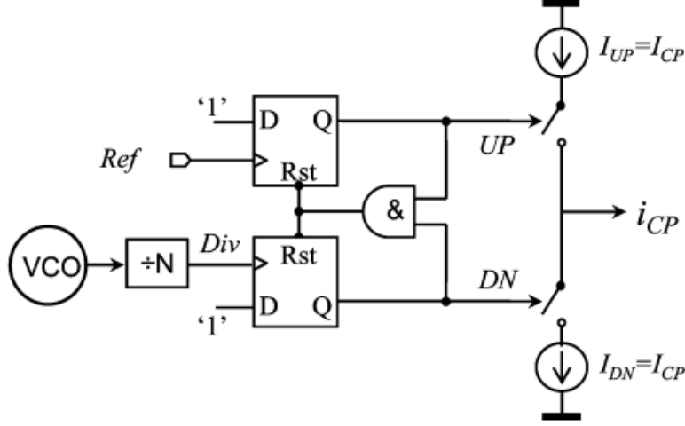
Figure 2.2: Commonly used tri-state PFD/CP (from [3])
