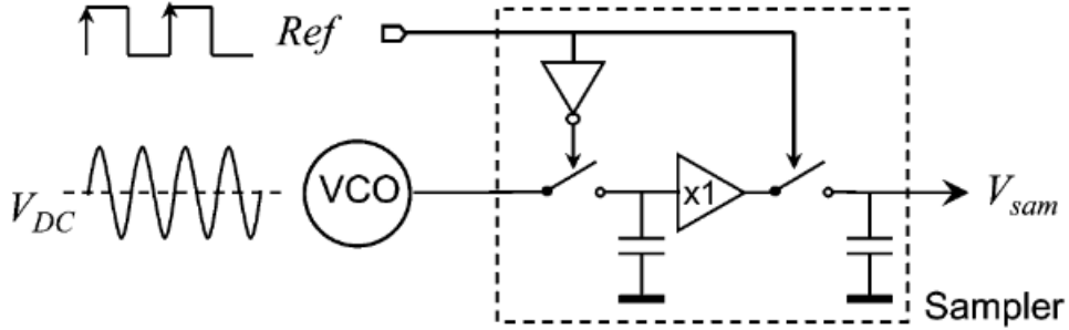
Figure 3.2: Conceptual diagram of sampling based PD [3]
