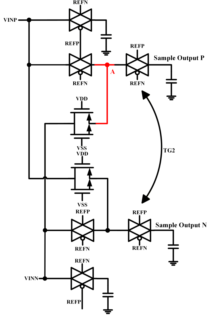
Figure 4.1: Circuit design of the SSPD
