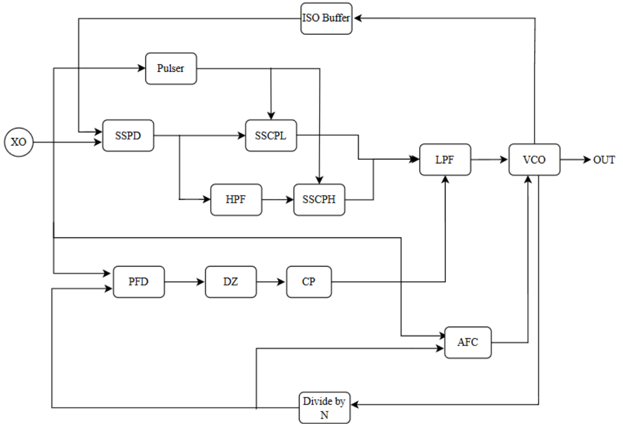
Figure 3.9: Block diagram of the proposed SSPLL
