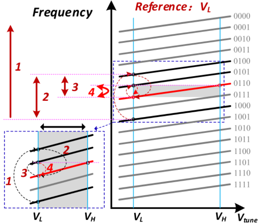
Figure 3.27: Search algorithm of the proposed O-AFC. [18]
