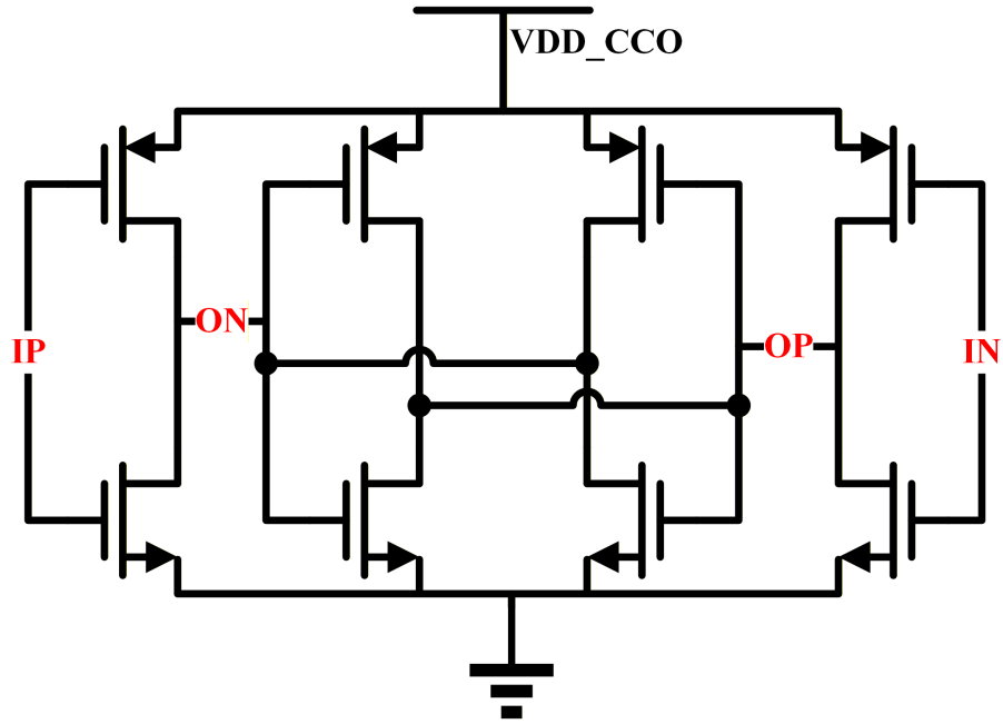
Figure 4.8: Circuit design of the CCO cell
