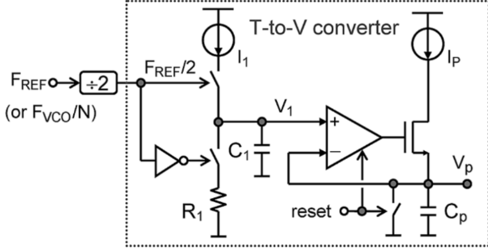
Figure 3.18: TVC circuit [17]
