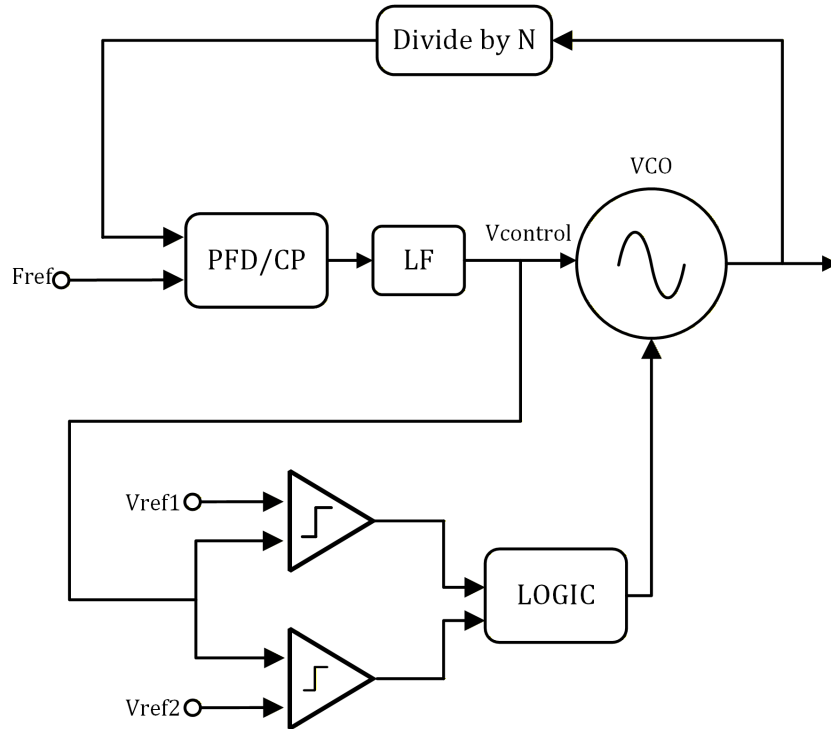
Figure 3.15: Conventional closed-loop VCO calibration technique
