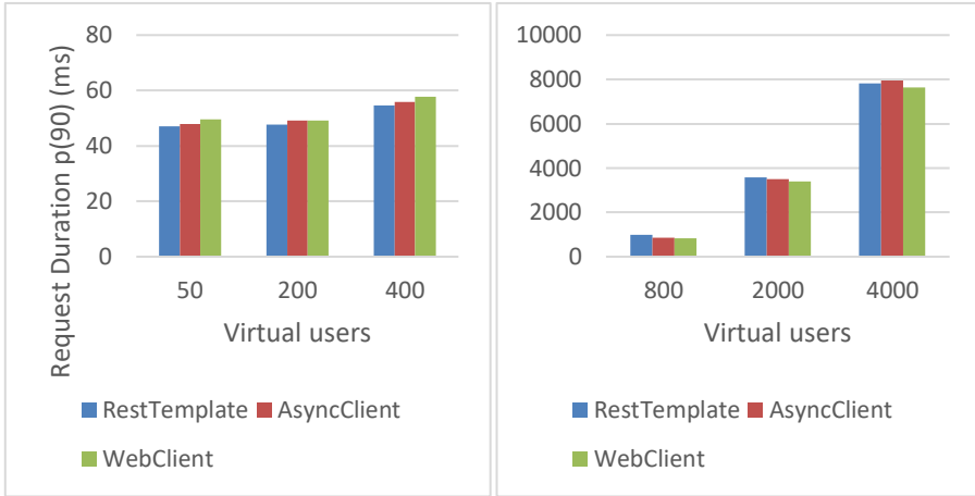
Fig. 30. Chart of the 90 th percentile request duration across varying numbers of virtual users
