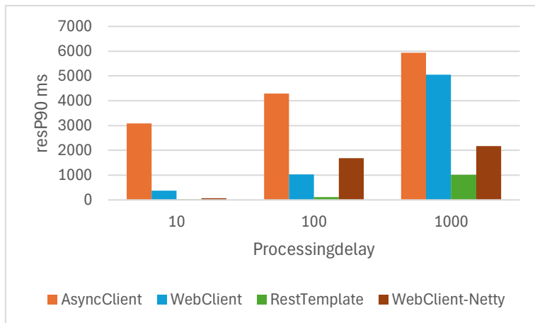
Fig. 18. Chart of response time in the 90 th percentile by length of processing delay in ms
