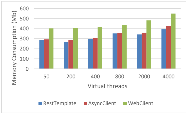
Fig. 32. Chart of memory consumption across varying numbers of virtual users
