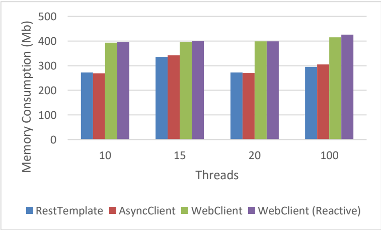
Fig. 36. Chart of memory consumption under constrained thread conditions
