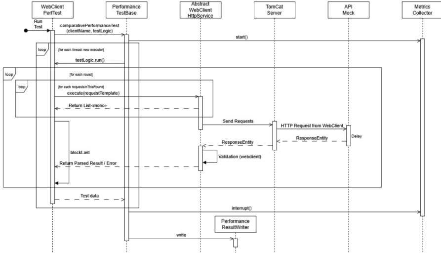
Fig. 3. WebClient local performance test
