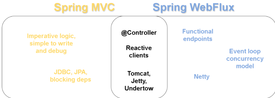
Fig. 1. Illustration of Spring MVC and Webflux and their differences, inspired by [4]
