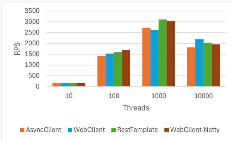
Fig. 13. Chart of RPS by number of threads
