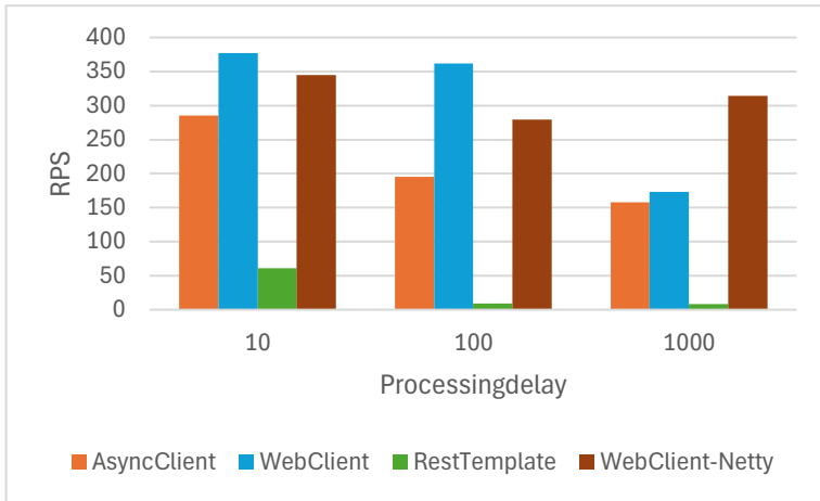
Fig. 17. Chart of RPS by length of processing delay in ms
