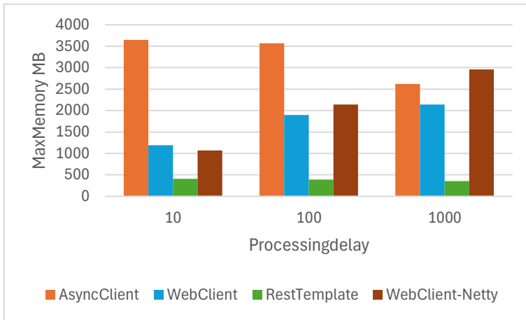
Fig. 20. Chart of maximum used memory by length of processing delay in ms
