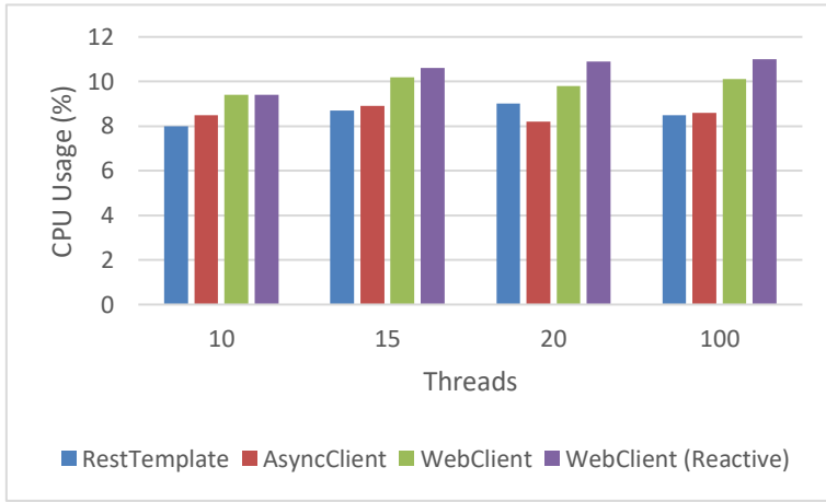
Fig. 37. Chart of CPU usage under constrained thread conditions
