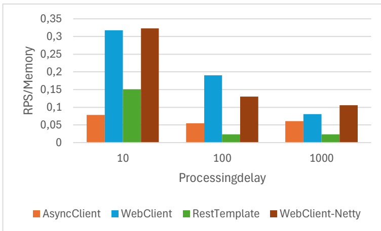
Fig. 21. Chart of RPS per MB of used memory
