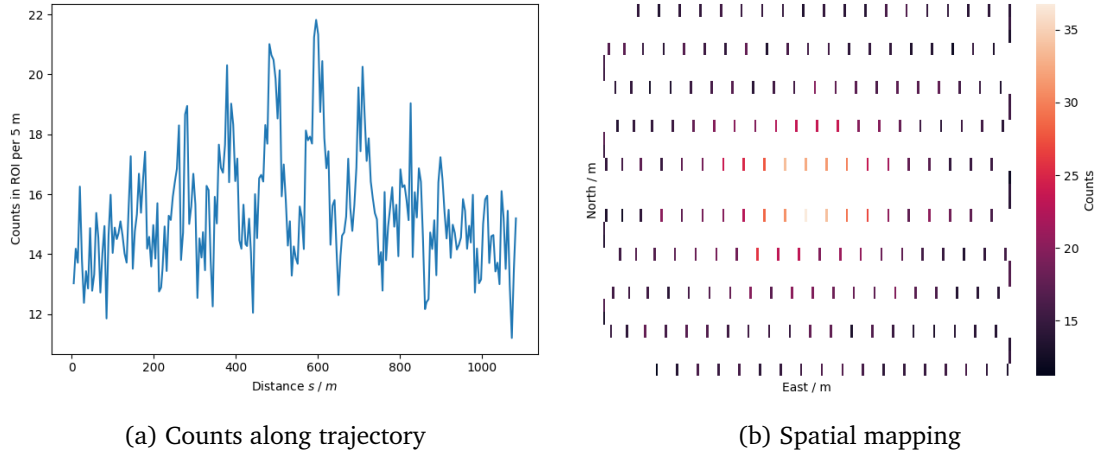
Figure 15: The counts along the trajectory at z = 15 m. This is the output directly generated by PG-RAD. b) Counts projected back to the (x, y) plane.
