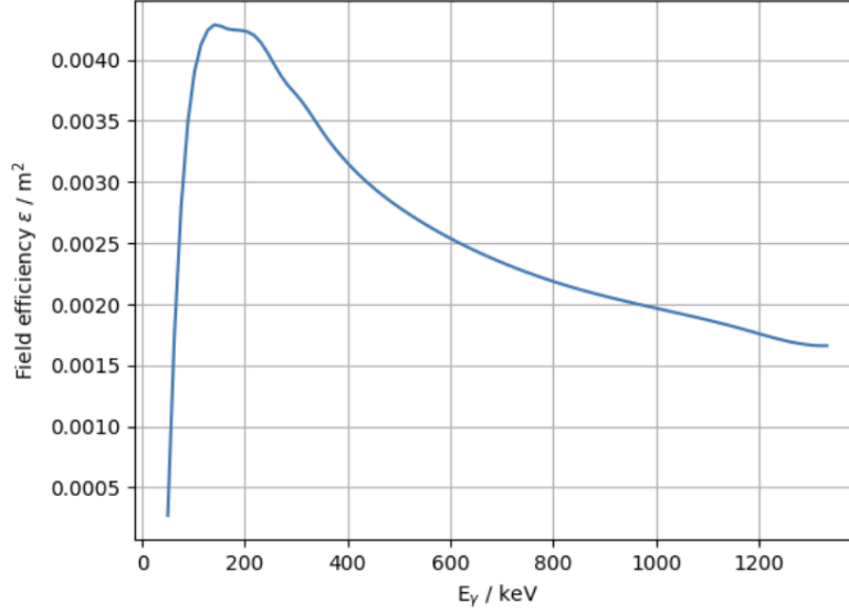
Figure 2: Field efficiency \epsilon_d(E_\gamma) of an HPGe detector mounted in a vehicle.
