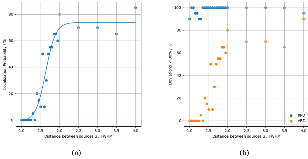
Figure 18: The localisation performance as a function of source separation d . The simulation used an HPGe detector travelling at 30 \text{ km h}^{-1} , measuring two 300 \text{ MBq } ^{137}\text{Cs} sources at 32 \text{ m} from the road. Figure a) shows the overall localisation probability (LP) as defined in Section 5.3.2. A sigmoidal fit is performed to the LP, which shows that the LP goes below 50% at a source separation of around 1.6 to 1.8 FWHM. Figure b) shows the percentage of scenarios with an ARD and RPD below 30% as a function of source separation d . The ARD is the dominant factor in a reduced LP at small source separations d . The RPD remains below the threshold, showing in this particular setup, the two-source algorithm continues to be able to locate the two sources, while the activity estimate becomes inaccurate.
