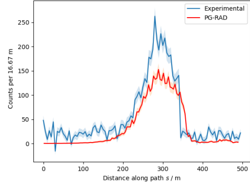
(b) “Setup 1”, NaI(Tl) (net counts)
