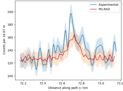
(c) “Road 2”, NaI(Tl) (gross counts)
