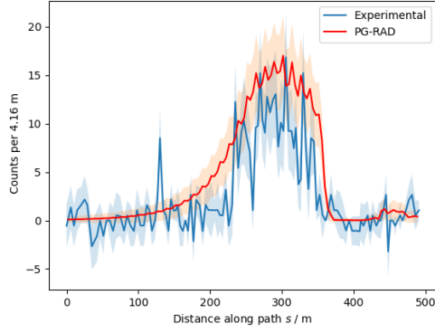
(a) “Setup 1”, HPGe (net counts)
