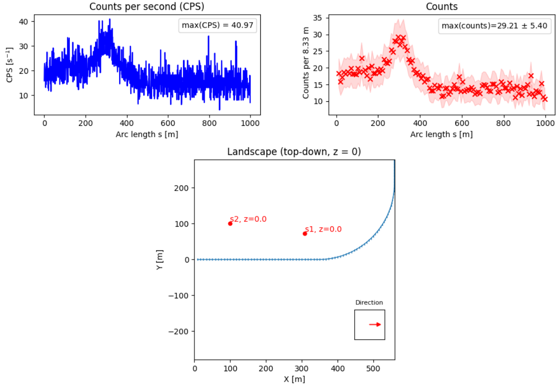
Figure 8: Plots produced by PG-RAD for the input shown in Listing 1. The top left figure shows the raw count rate along the trajectory. The top right shows the integrated count rates. With an acquisition time of 1 s and a velocity of 8.33 \text{ m s}^{-1} , the road is segmented into 8.33 m bins. Note that the integrated counts after 1 second acquisition time are lower than the maximum of the count rate function. This has to do with alignment of integration windows as shown in Figure 6. The bottom figure shows a top-down visualisation of the scenario.
