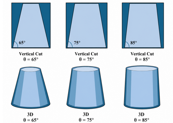
Figure 3.9: Vertical cross-sectional and three-dimensional illustrations of conical microvias with sidewall angles of \theta = 65^\circ , 75^\circ , and 85^\circ . A smaller angle indicates a stronger tapering effect, while a larger angle approaches the cylindrical-via limit.
