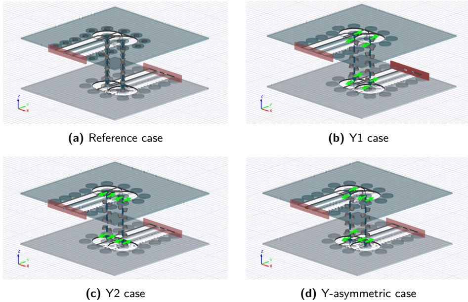
Figure 4.3: Three-dimensional dimetric views of the y -direction hole misalignment cases. The ground vias and ground layers are hidden for clarity. The dark-blue solid lines show the fan-in and fan-out directions on layers 3 and 15. The green arrows mark the hole offsets along the y -direction.
