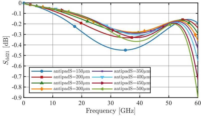
(b) Layer 3 to Layer 9 transition;
