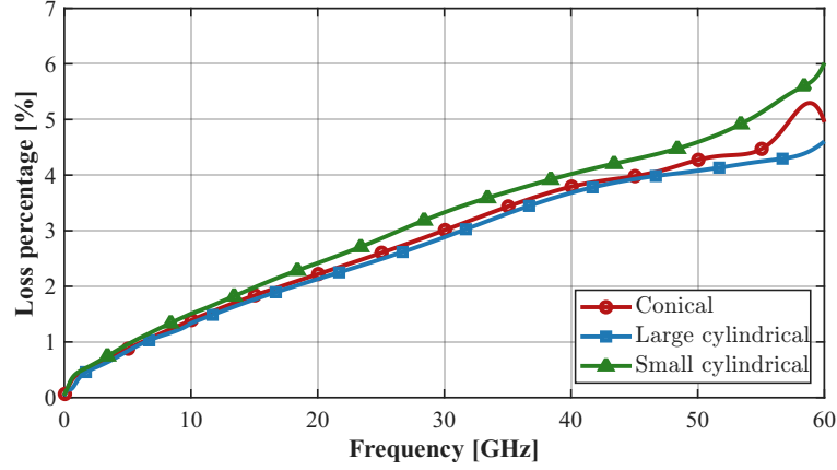
Figure 3.20: Estimated radiation-related loss percentage for the L3–L15 transition structure using different microvia geometry models.
