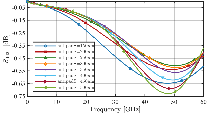
(a) Layer 3 to Layer 7 transition;
